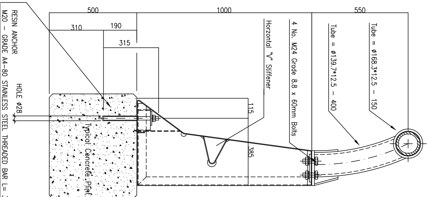
Cross Section of Sistema Barrier Showing Typical Anchor Detail
